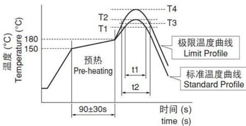
回流焊温度曲线 Reflow Soldering Temperature Profile
